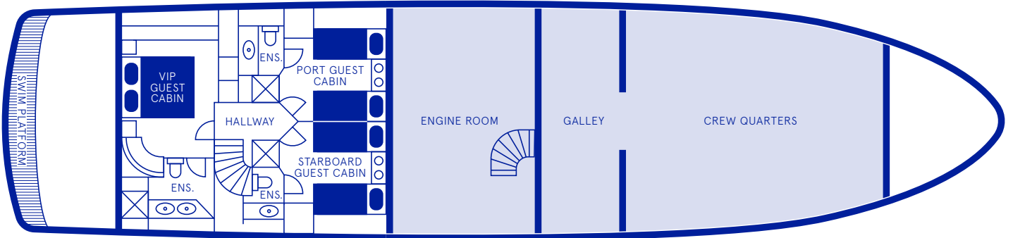
CABIN DECK (OPTION 1)
